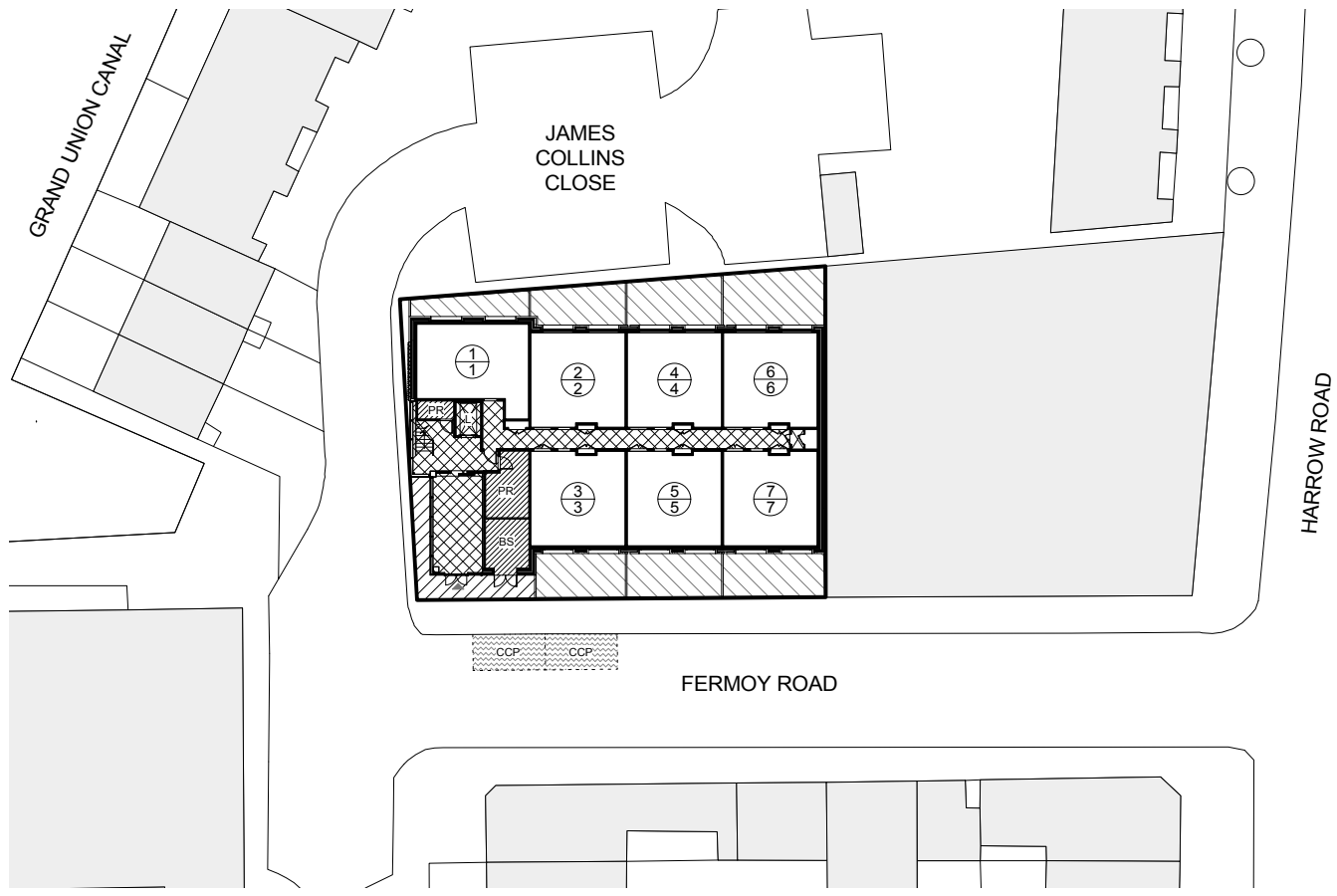
SITE PLAN & GROUND FLOOR
